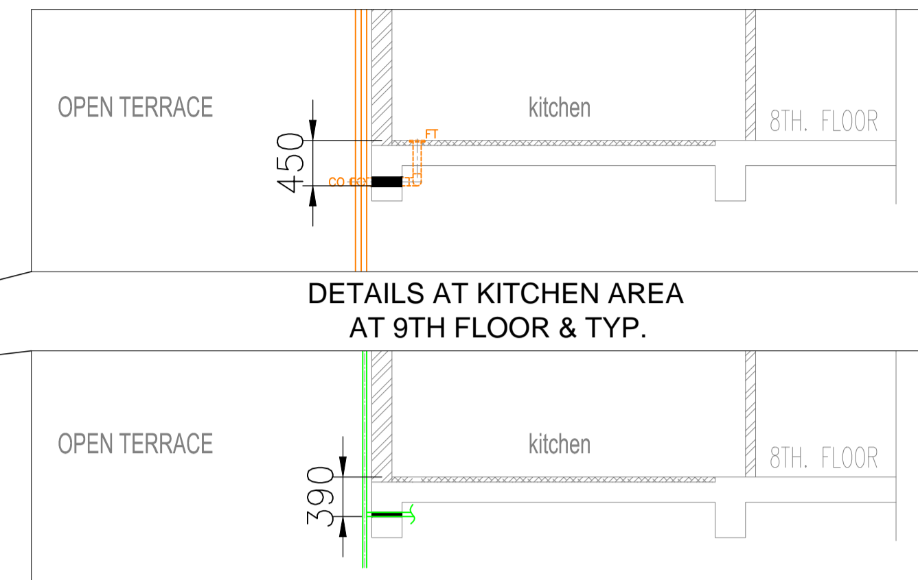
DETAILS AT KITCHEN AREA AT 9TH FLOOR & TYP.
