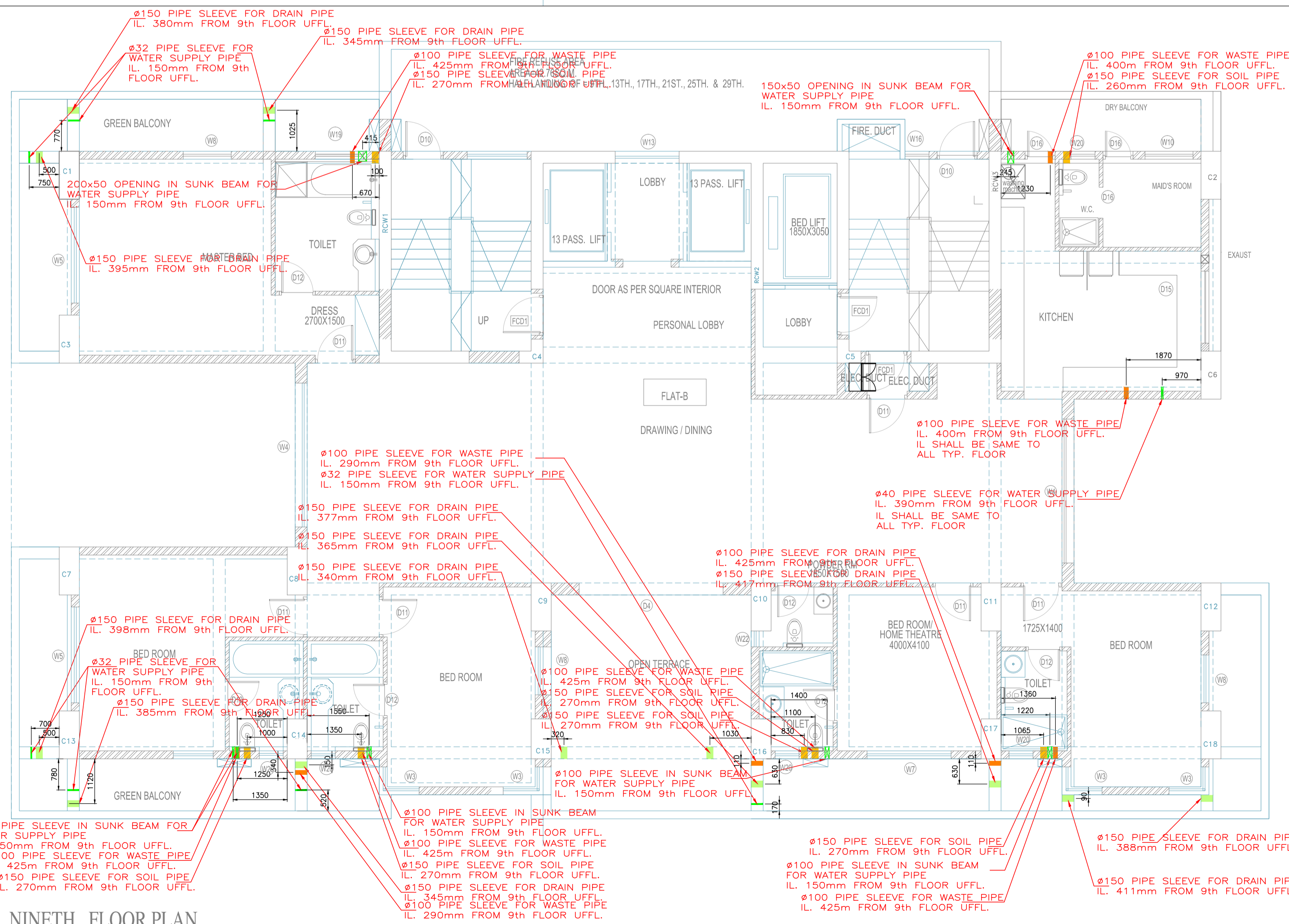
NINETH FLOOR PLAN
